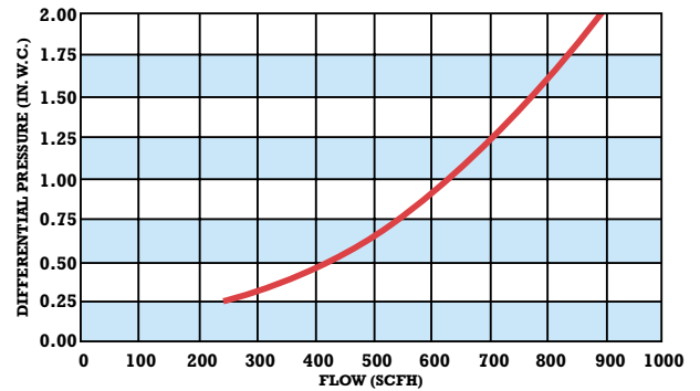
AL-425 CAPACITY CURVE @ .25 PSIG inlet
